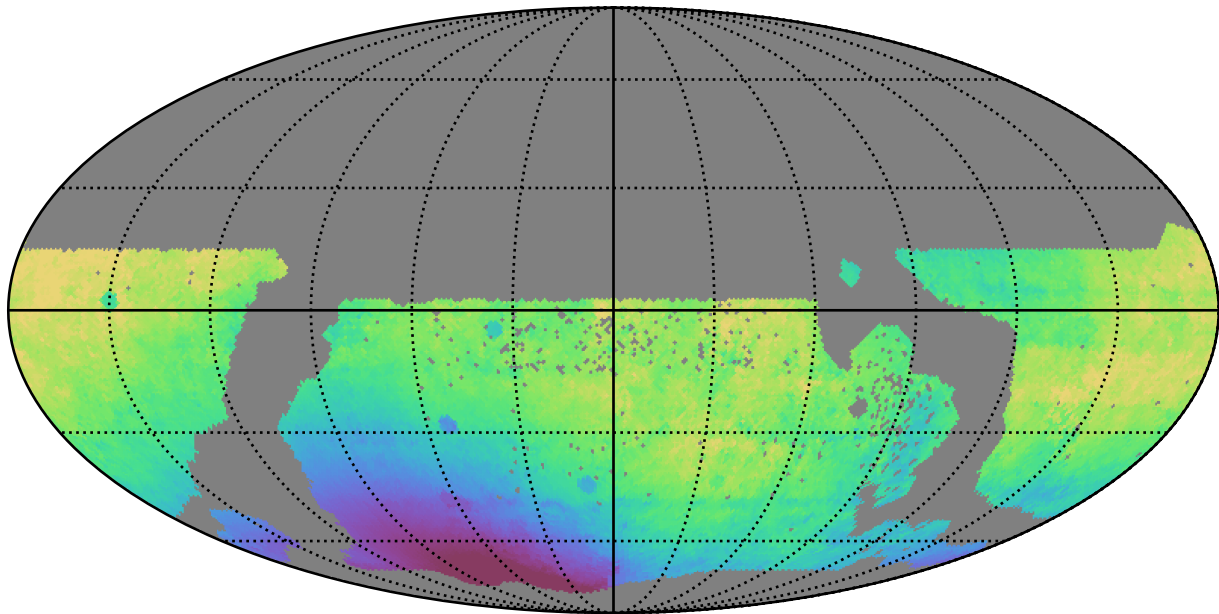
too_100_1v3.4_10yrs WFD r band: Median solarElong
