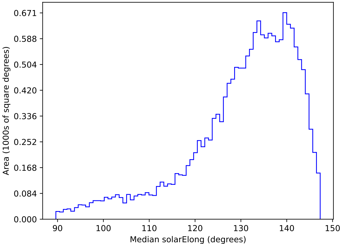
too_100_1v3.4_10yrs WFD r band: Median solarElong
