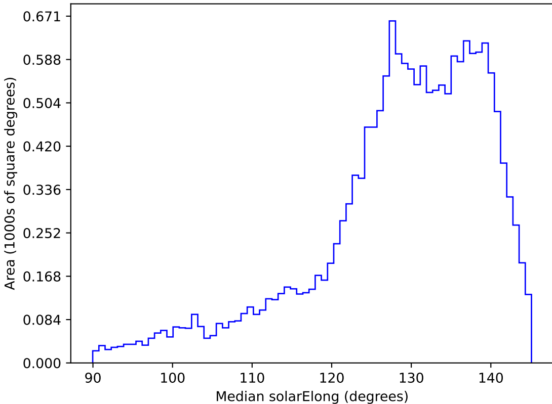
too_100_1v3.4_10yrs WFD i band: Median solarElong
