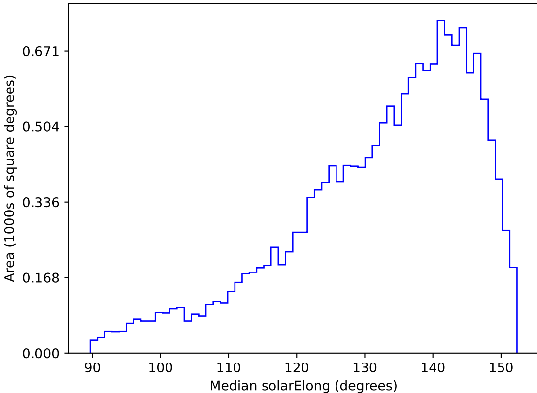
too_100_1v3.4_10yrs WFD g band: Median solarElong
