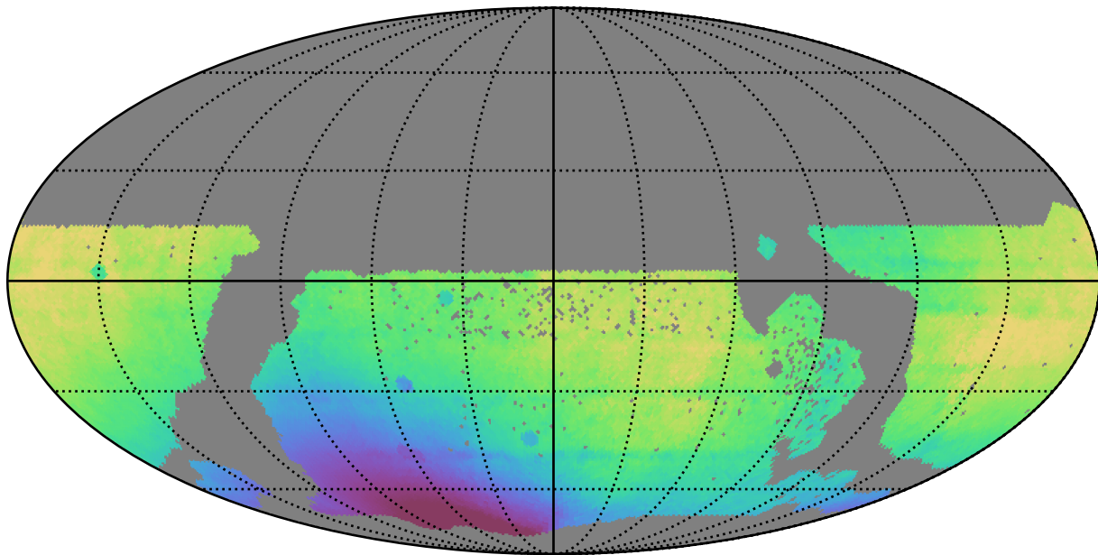
too_100_1v3.4_10yrs WFD all bands: Median solarElong
