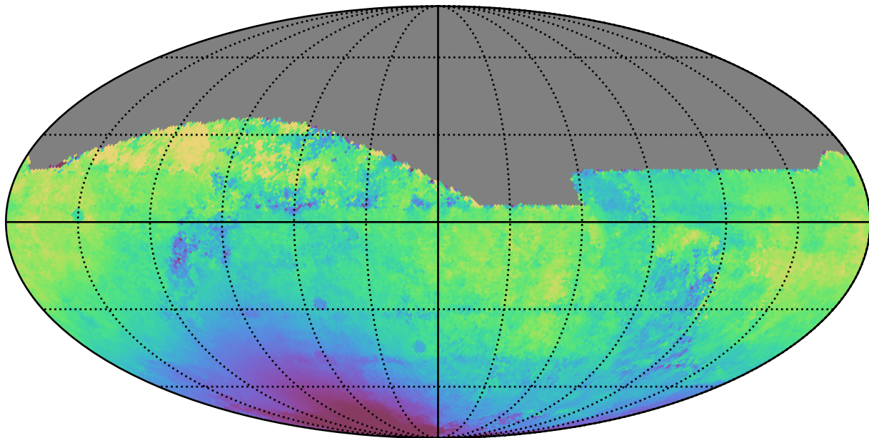
too_100_1v3.4_10yrs All sky z band: Median solarElong
