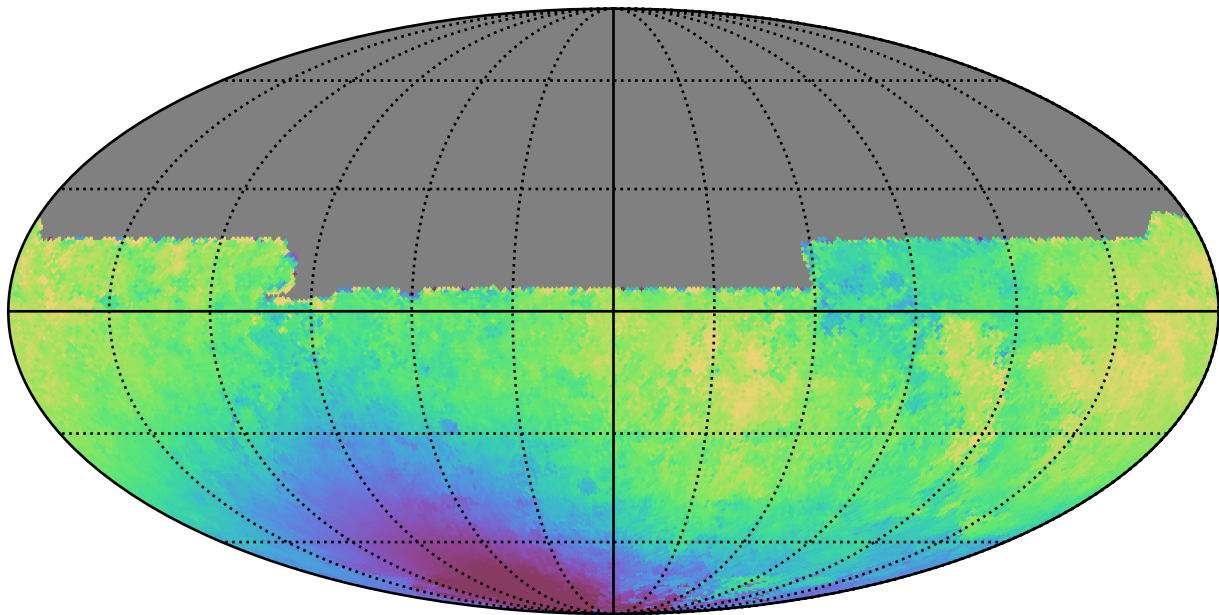
too_100_1v3.4_10yrs All sky y band: Median solarElong
