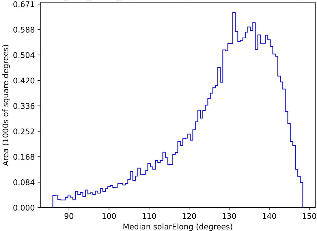
too_100_1v3.4_10yrs All sky y band: Median solarElong
