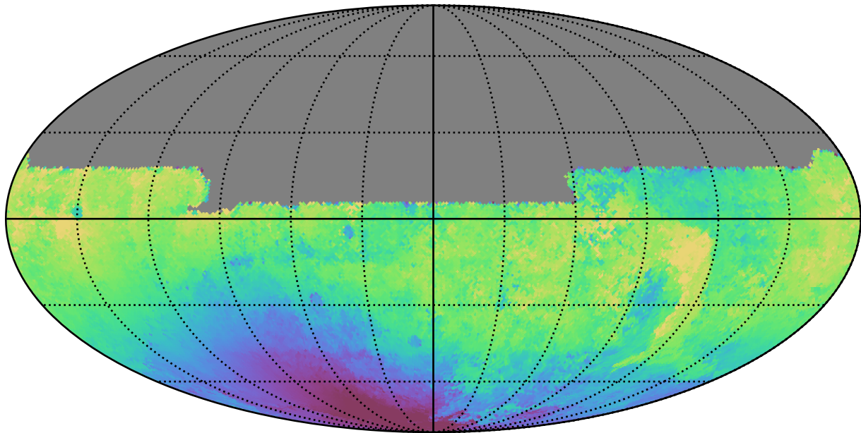
too_100_1v3.4_10yrs All sky u band: Median solarElong
