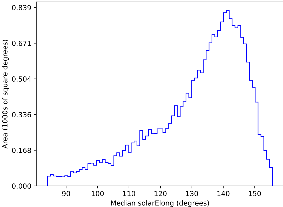
too_100_1v3.4_10yrs All sky u band: Median solarElong
