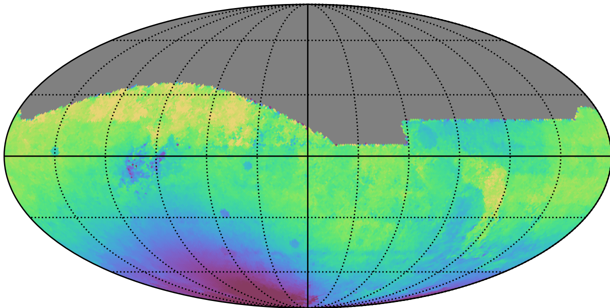
too_100_1v3.4_10yrs All sky r band: Median solarElong
