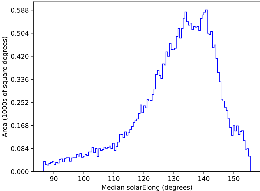
too_100_1v3.4_10yrs All sky r band: Median solarElong
