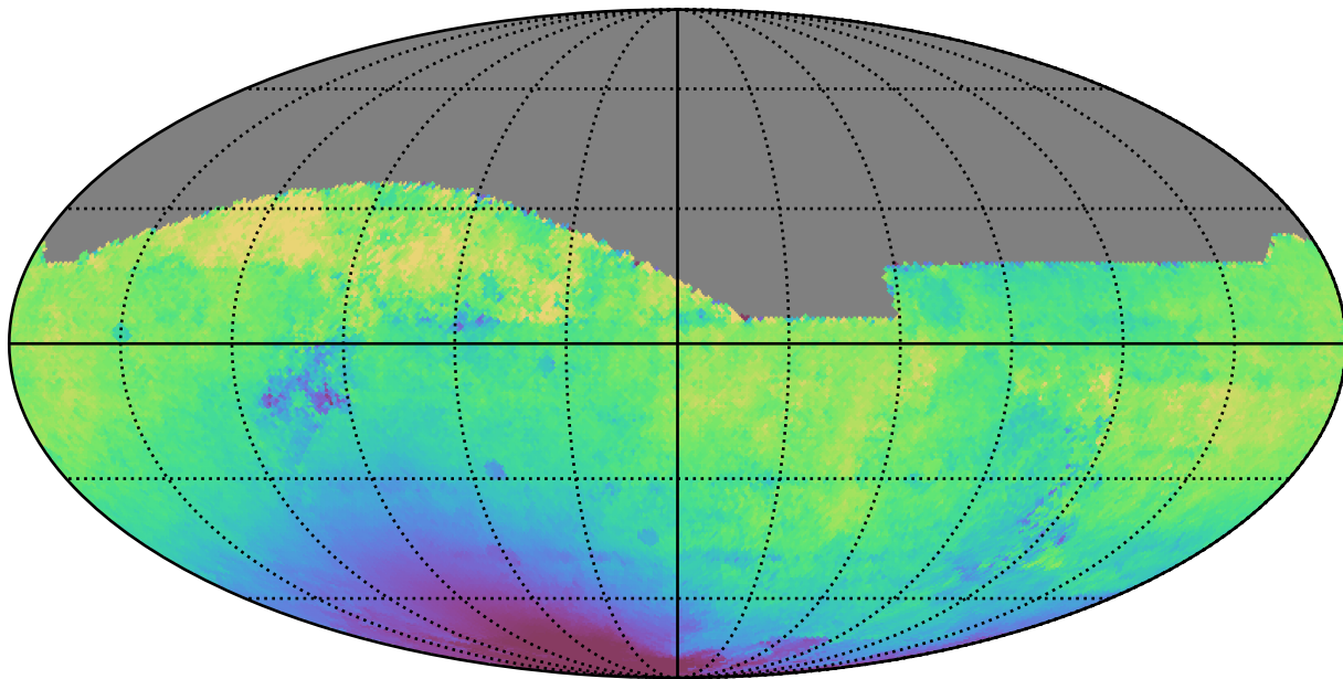
too_100_1v3.4_10yrs All sky i band: Median solarElong
