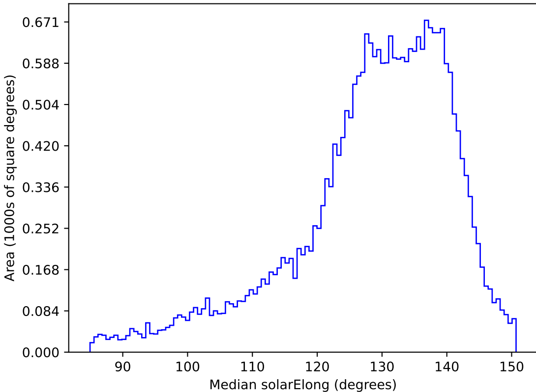
too_100_1v3.4_10yrs All sky i band: Median solarElong
