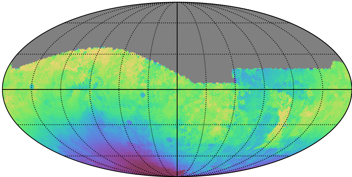
too_100_1v3.4_10yrs All sky g band: Median solarElong
