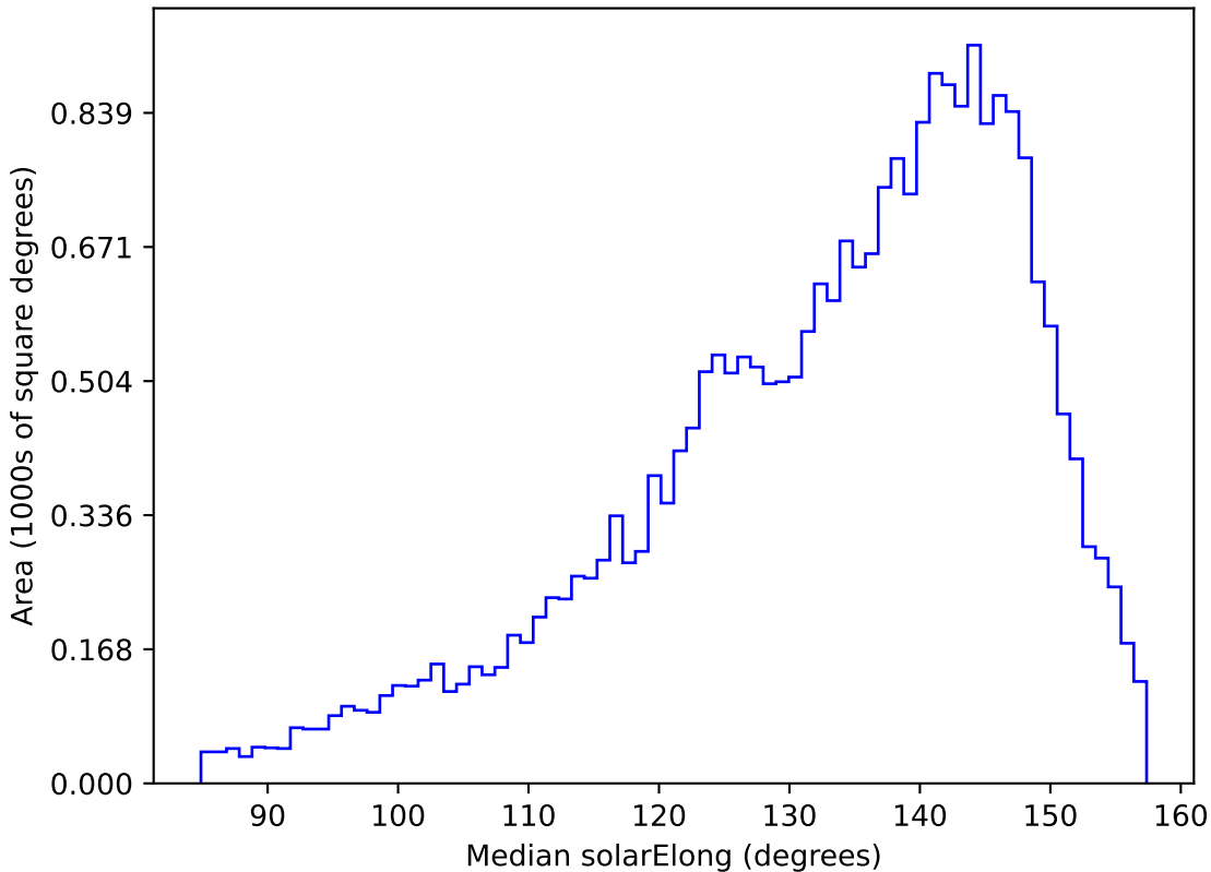
too_100_1v3.4_10yrs All sky g band: Median solarElong
