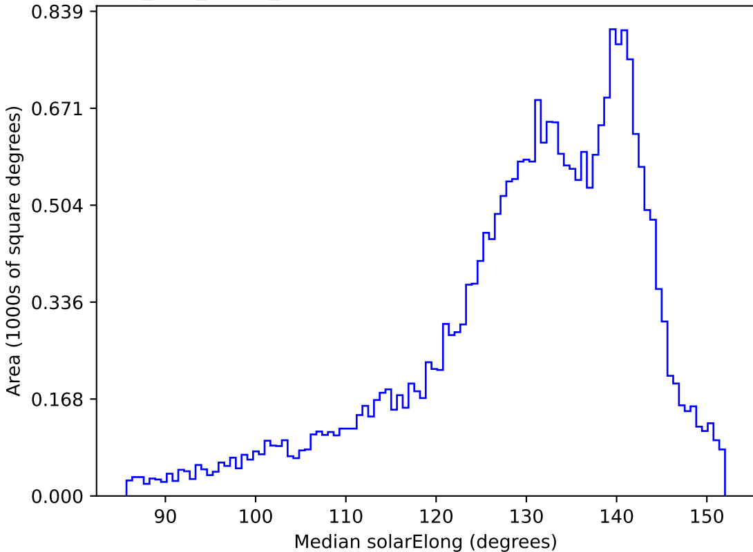
too_100_1v3.4_10yrs All sky all bands: Median solarElong
