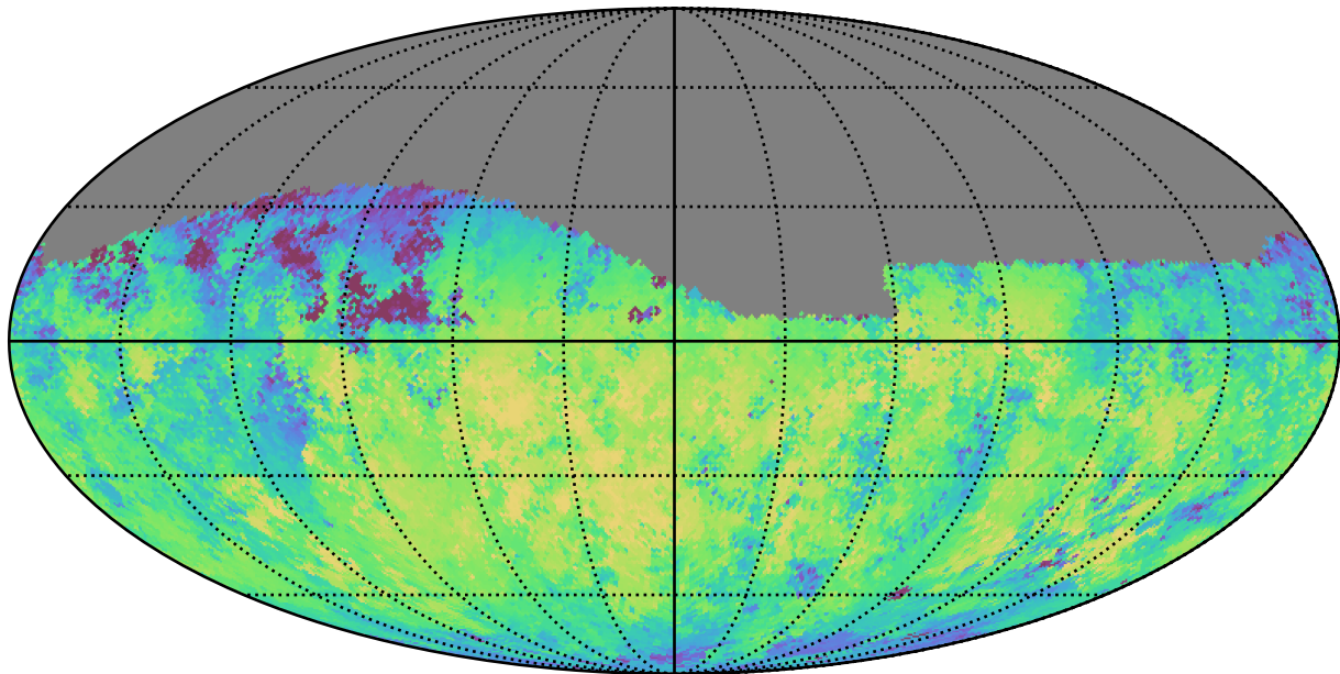
too_100_1v3.4_10yrs Yr 1 z band: Median skyBrightness
