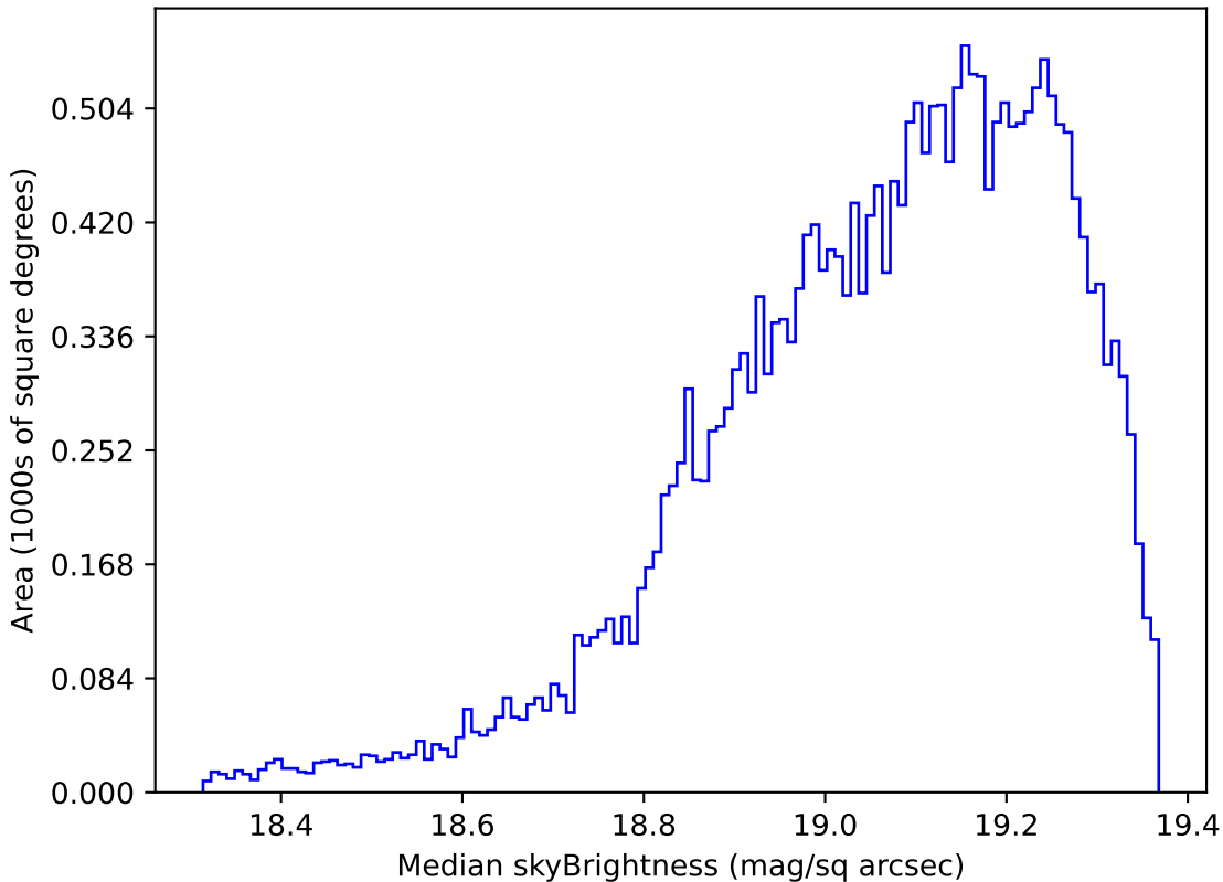
too_100_1v3.4_10yrs Yr 1 z band: Median skyBrightness
