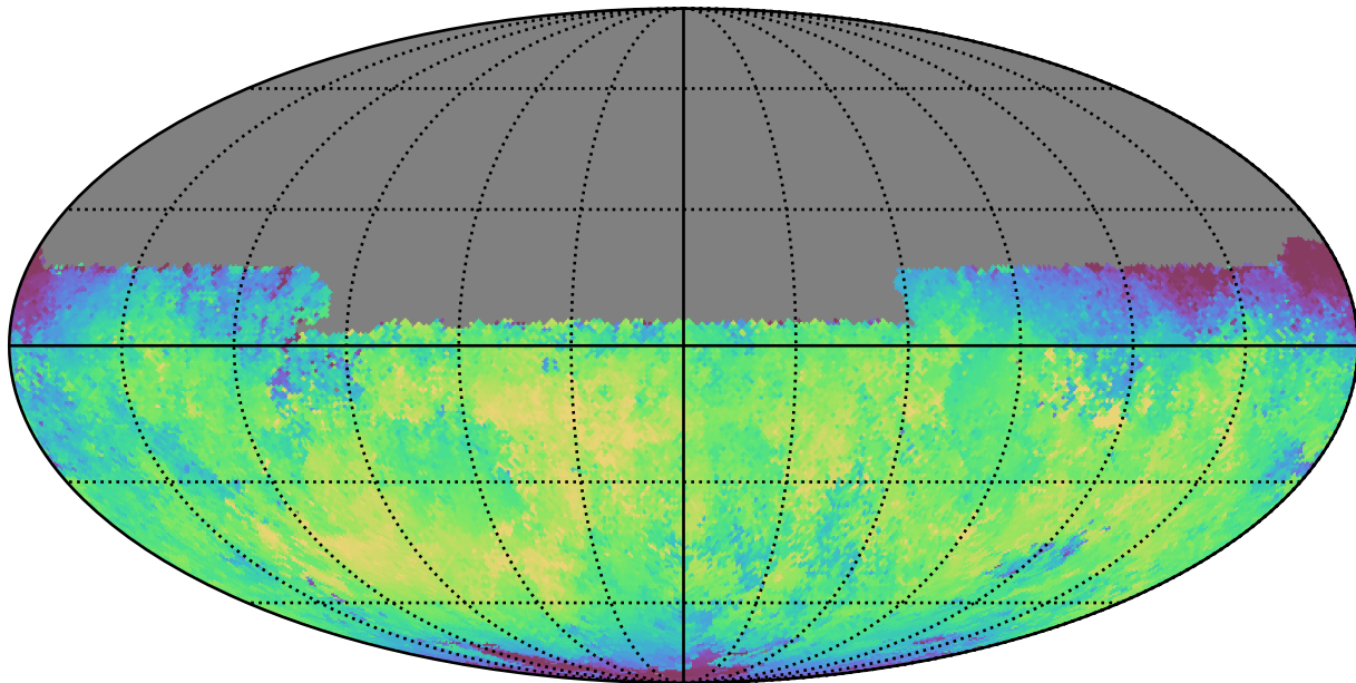
too_100_1v3.4_10yrs Yr 1 y band: Median skyBrightness
