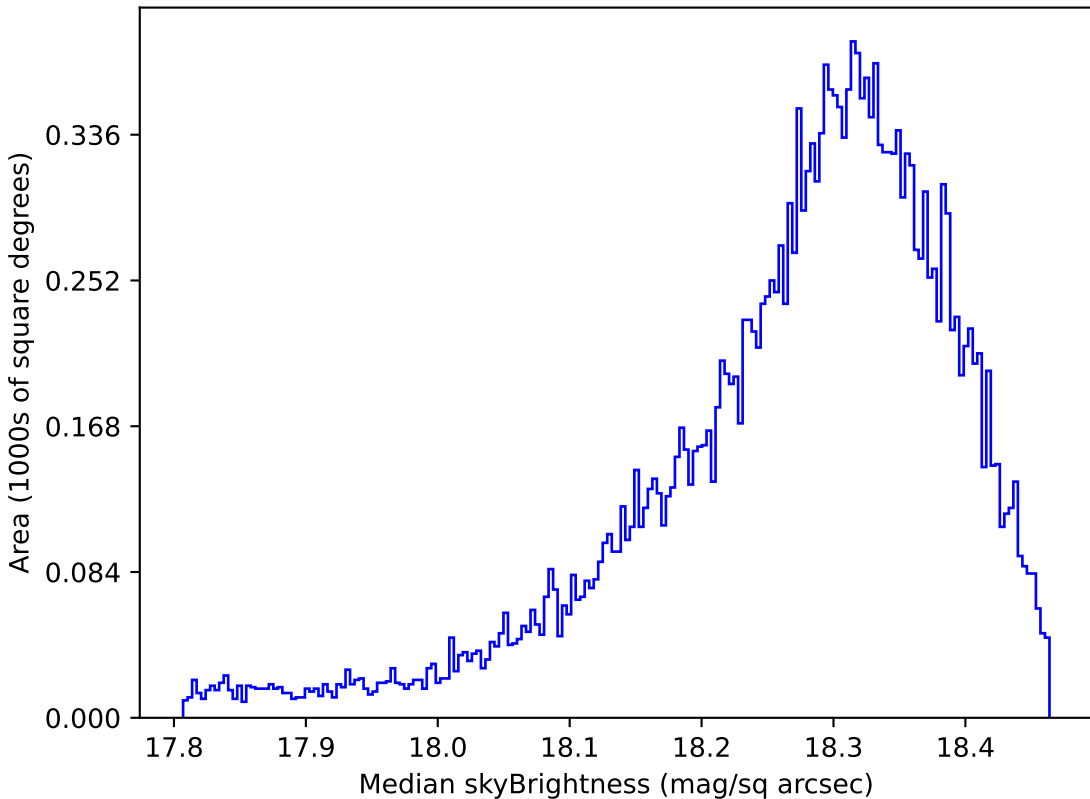
too_100_1v3.4_10yrs Yr 1 y band: Median skyBrightness
