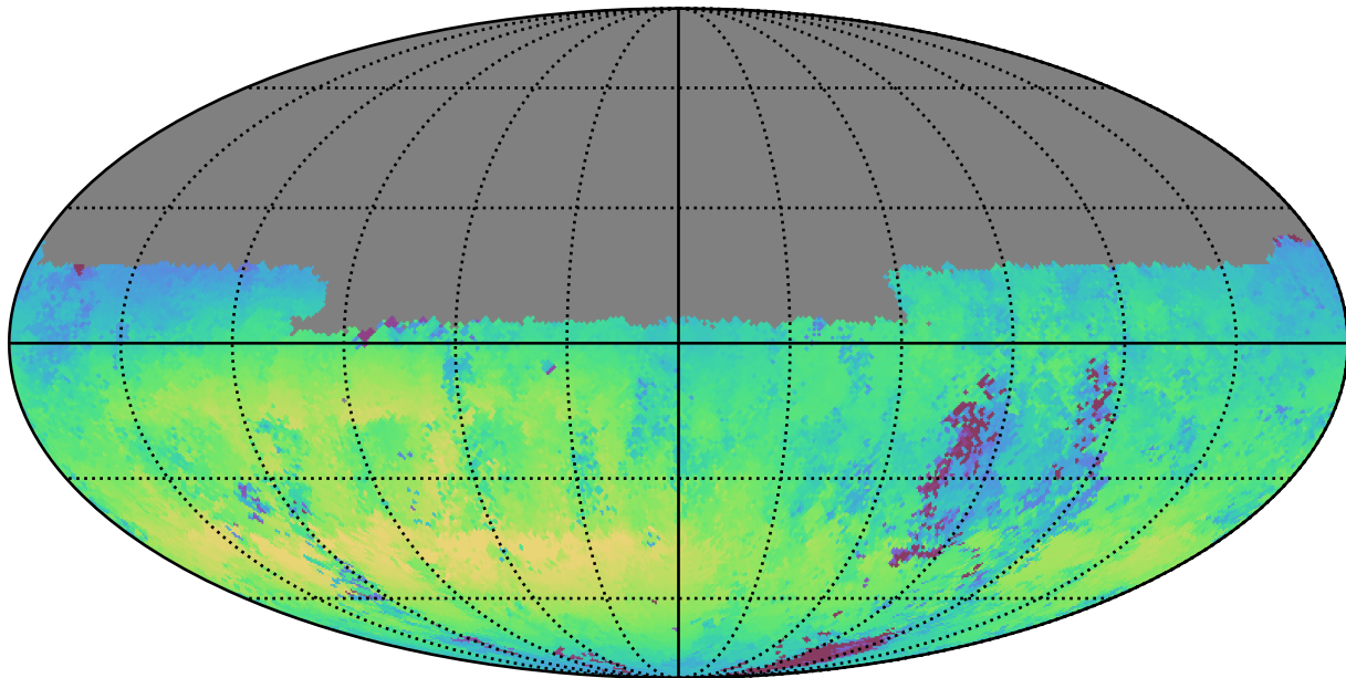
too_100_1v3.4_10yrs Yr 1 u band: Median skyBrightness
