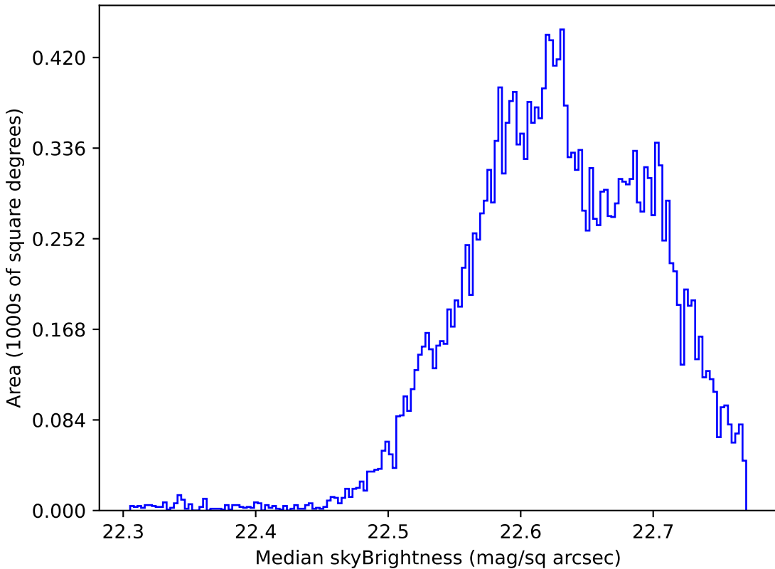
too_100_1v3.4_10yrs Yr 1 u band: Median skyBrightness
