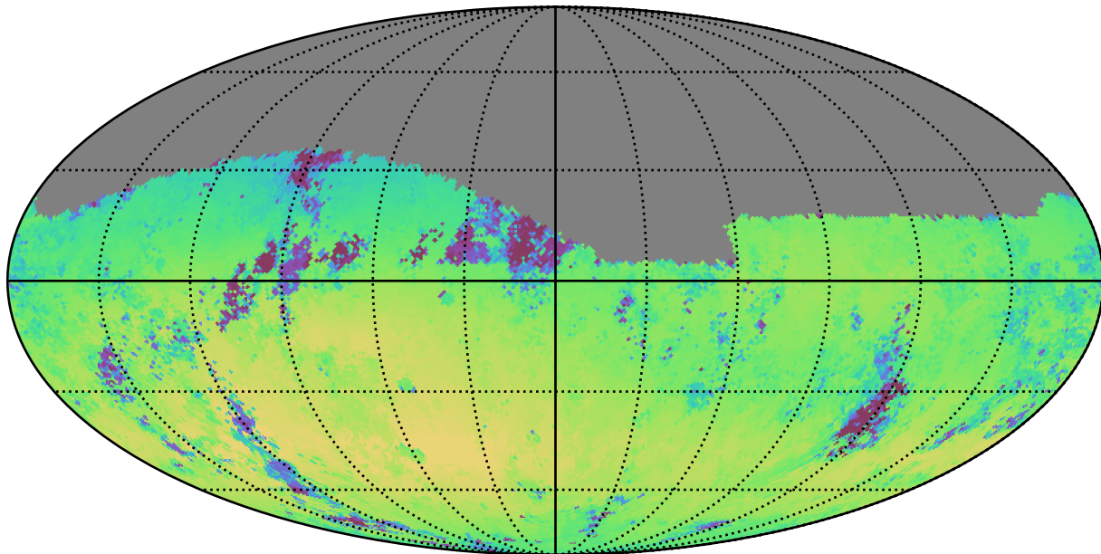
too_100_1v3.4_10yrs Yr 1 r band: Median skyBrightness
