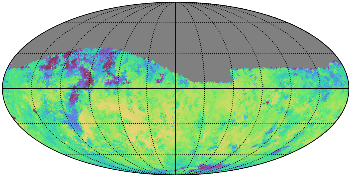
too_100_1v3.4_10yrs Yr 1 i band: Median skyBrightness
