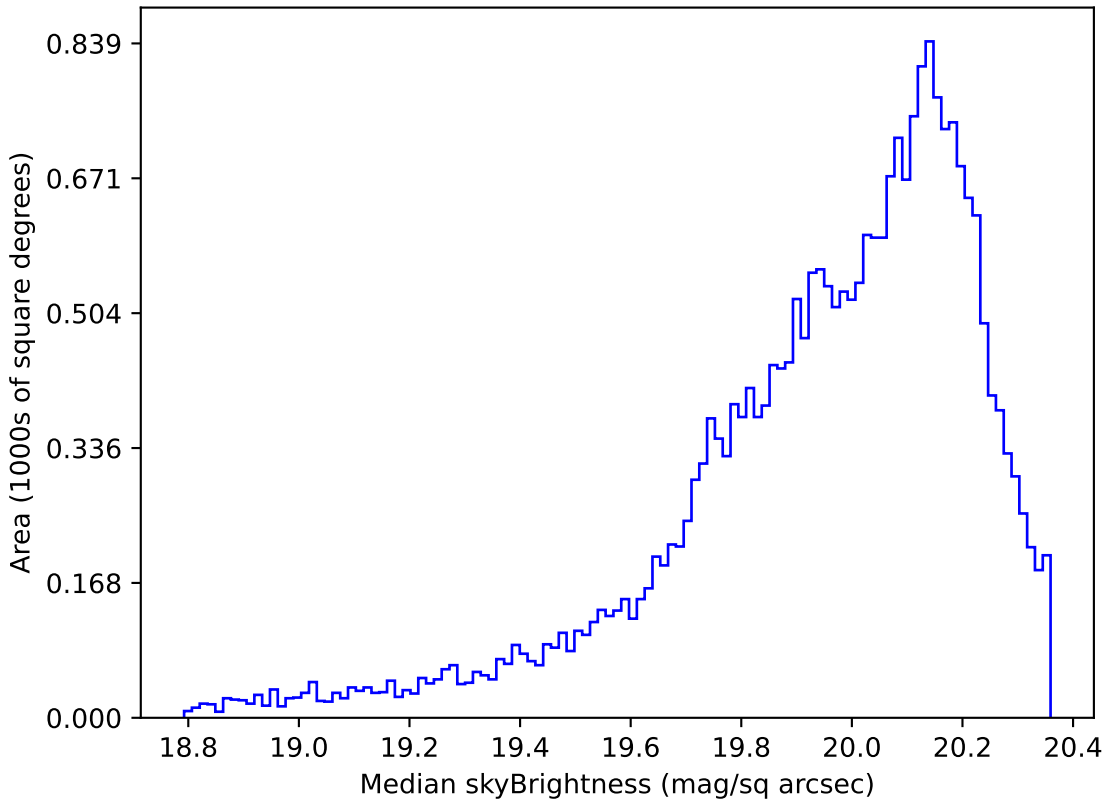
too_100_1v3.4_10yrs Yr 1 i band: Median skyBrightness
