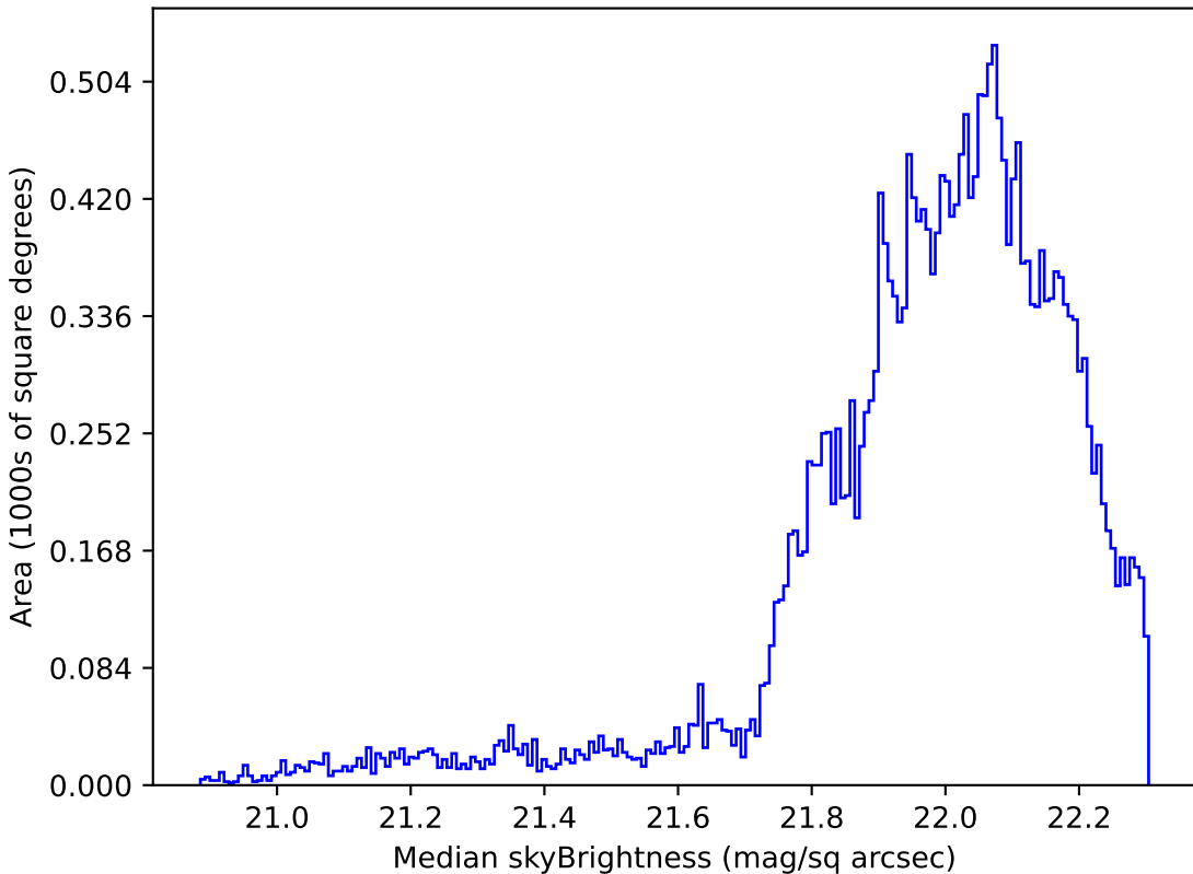
too_100_1v3.4_10yrs Yr 1 g band: Median skyBrightness
