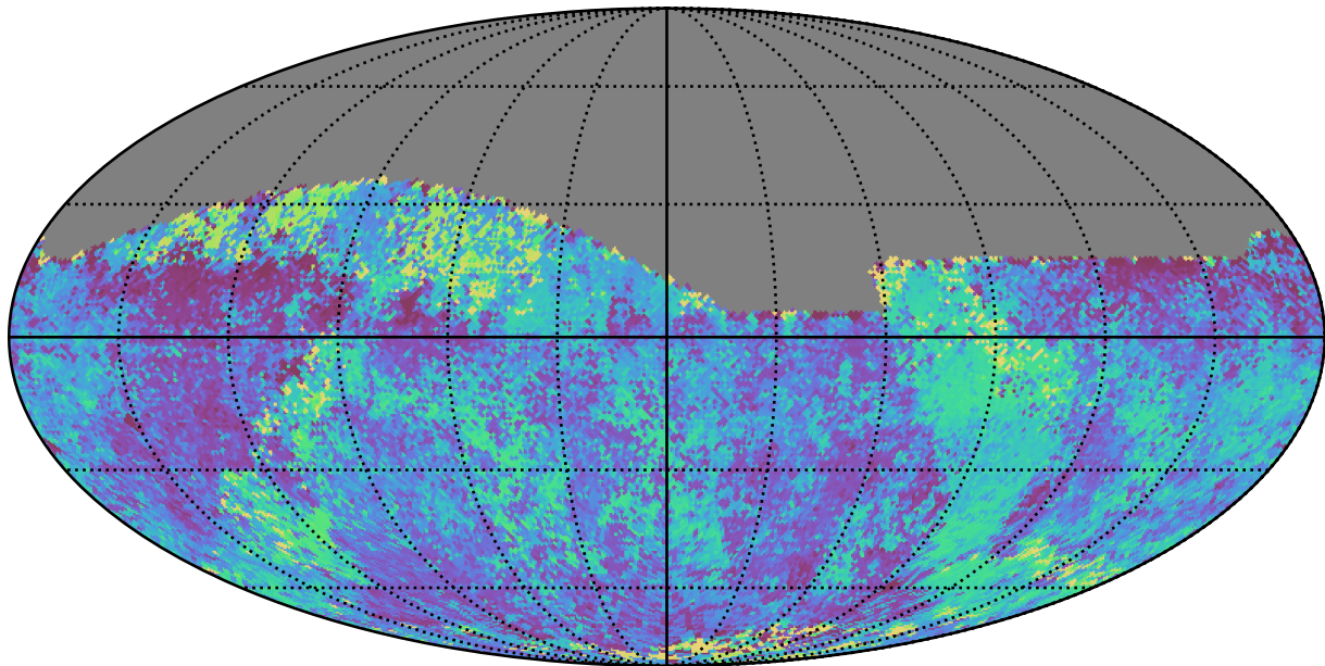
too_100_1v3.4_10yrs Yr 1 all bands: Median skyBrightness
