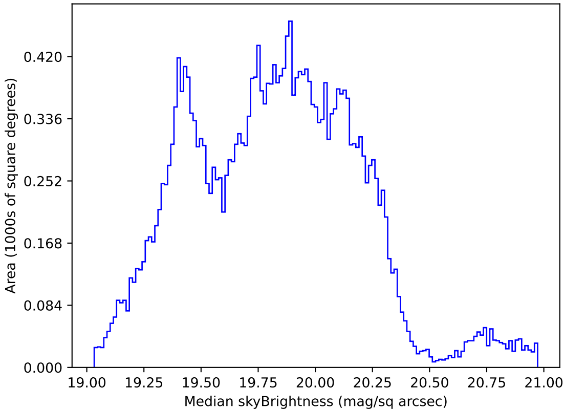
too_100_1v3.4_10yrs Yr 1 all bands: Median skyBrightness
