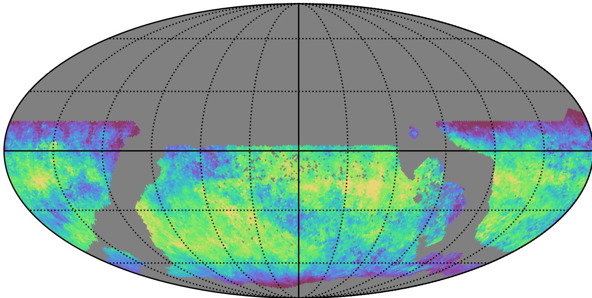
too_100_1v3.4_10yrs WFD z band: Median skyBrightness
