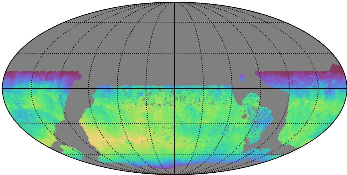
too_100_1v3.4_10yrs WFD y band: Median skyBrightness
