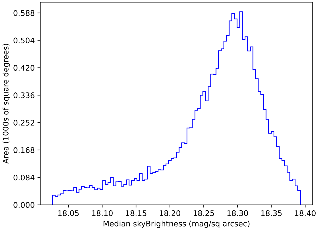
too_100_1v3.4_10yrs WFD y band: Median skyBrightness
