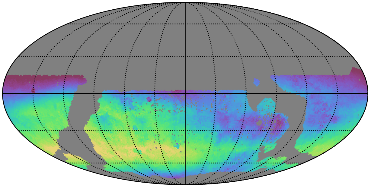
too_100_1v3.4_10yrs WFD u band: Median skyBrightness
