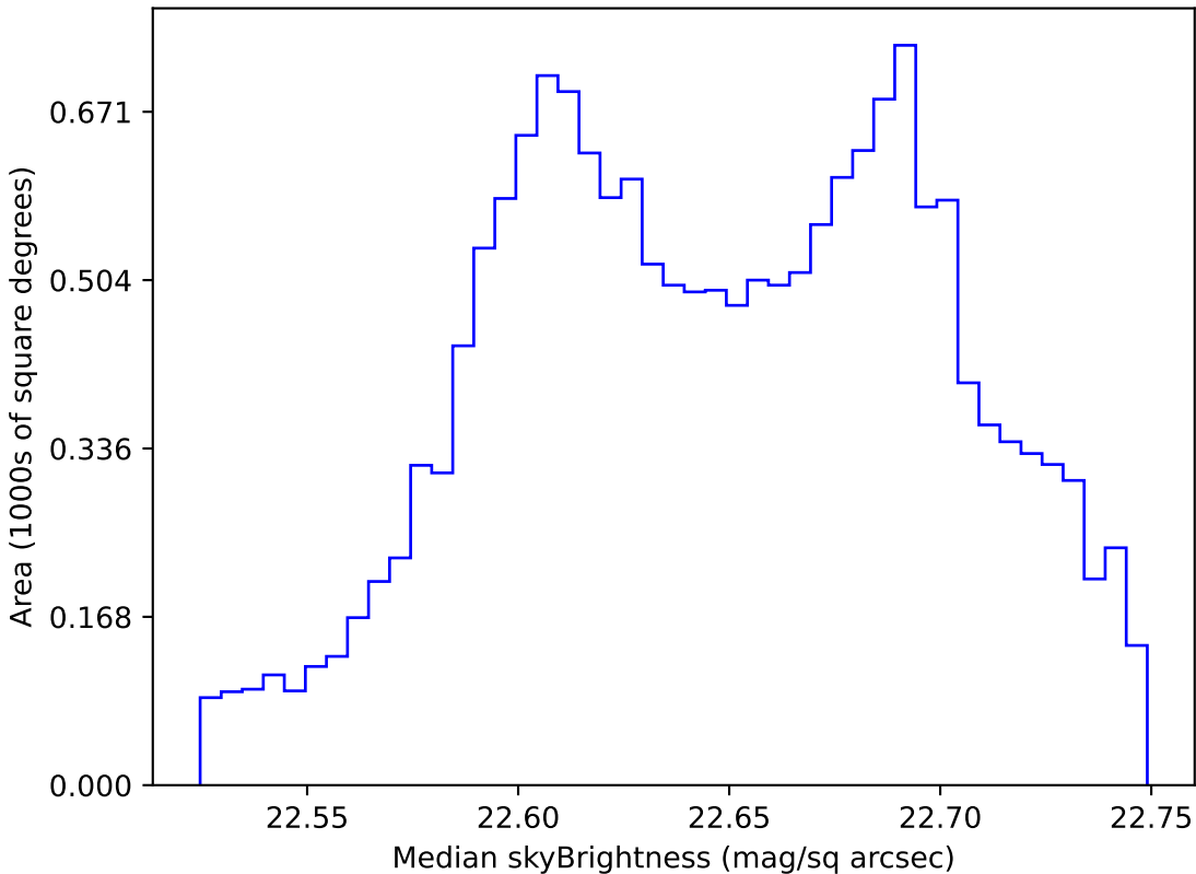
too_100_1v3.4_10yrs WFD u band: Median skyBrightness
