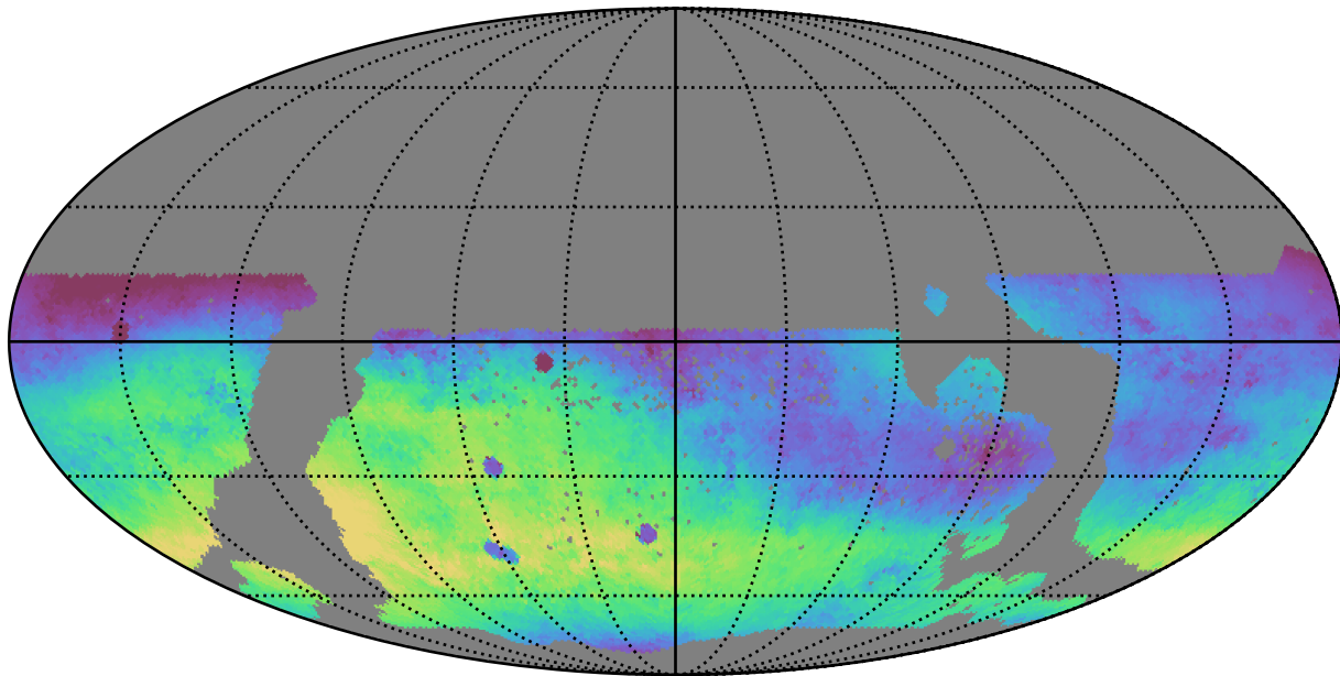
too_100_1v3.4_10yrs WFD r band: Median skyBrightness
