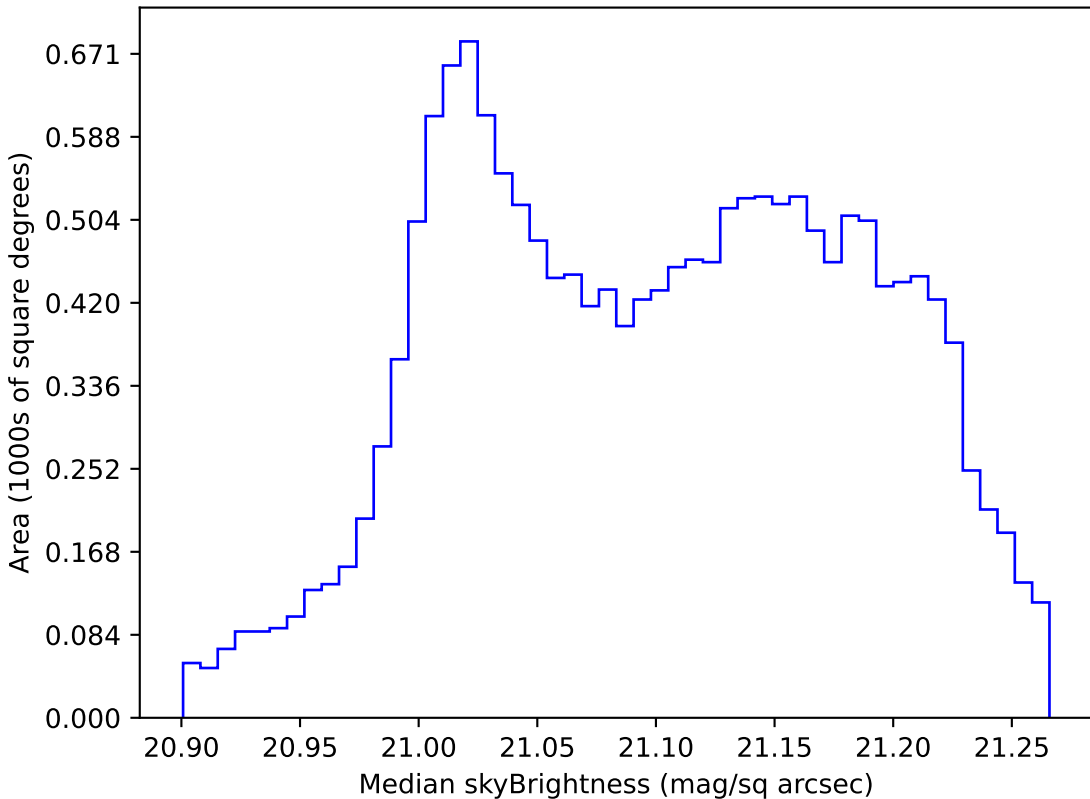
too_100_1v3.4_10yrs WFD r band: Median skyBrightness
