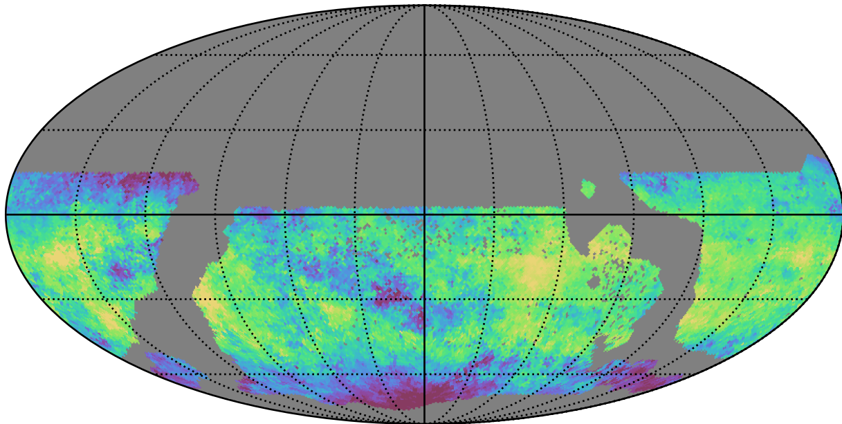
too_100_1v3.4_10yrs WFD i band: Median skyBrightness
