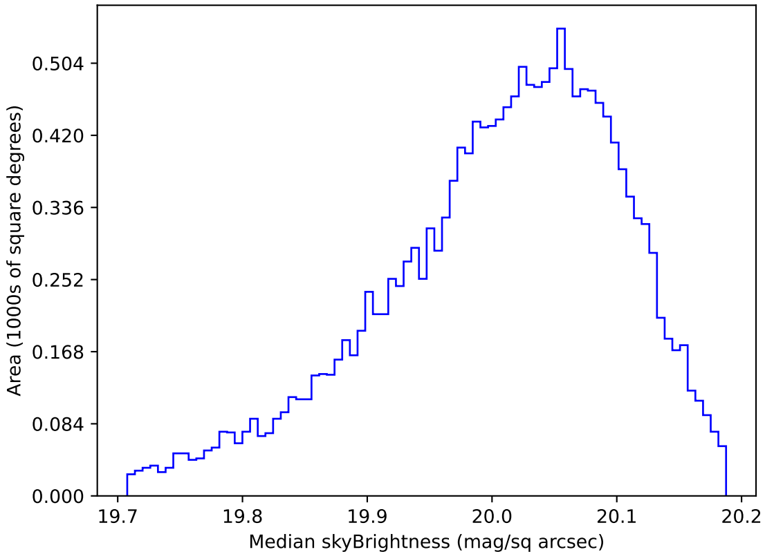
too_100_1v3.4_10yrs WFD i band: Median skyBrightness
