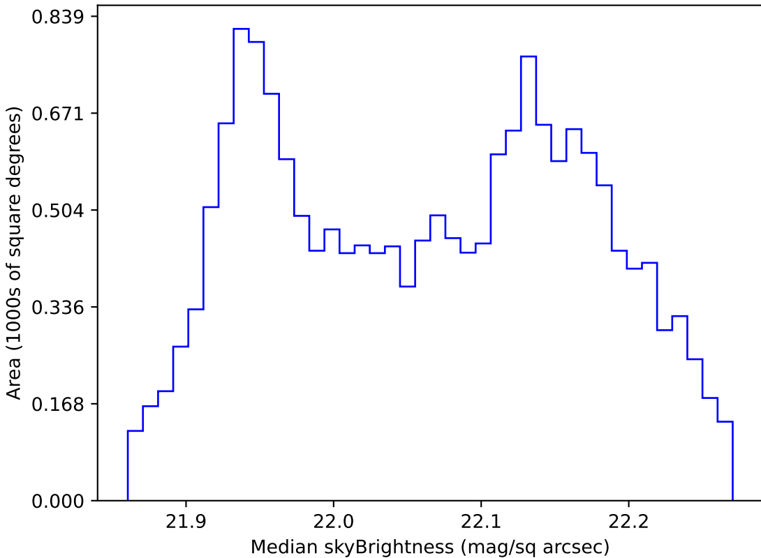
too_100_1v3.4_10yrs WFD g band: Median skyBrightness
