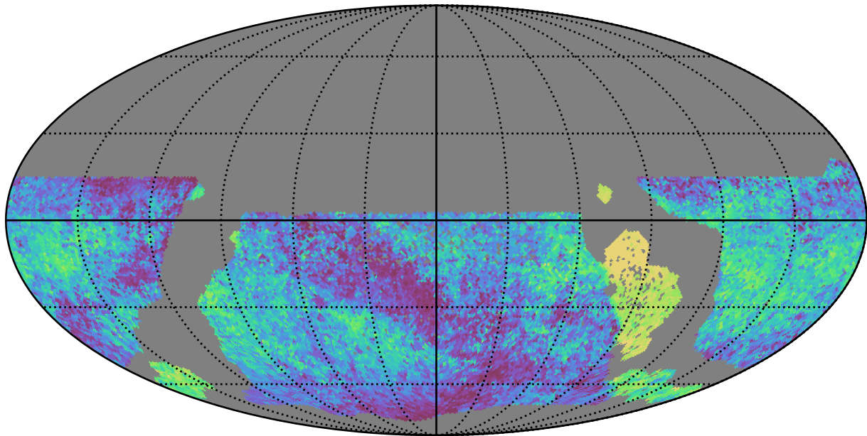
too_100_1v3.4_10yrs WFD all bands: Median skyBrightness
