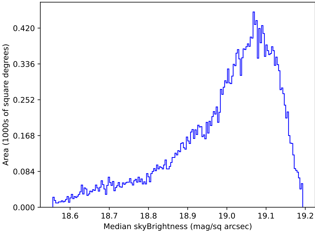
too_100_1v3.4_10yrs All sky z band: Median skyBrightness
