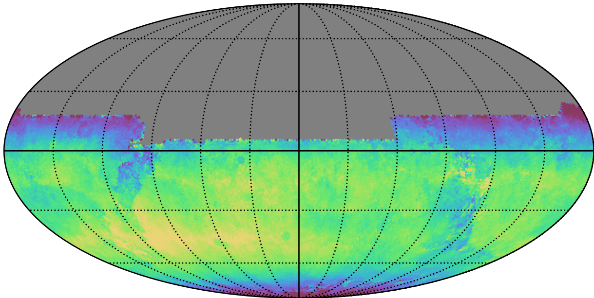
too_100_1v3.4_10yrs All sky y band: Median skyBrightness
