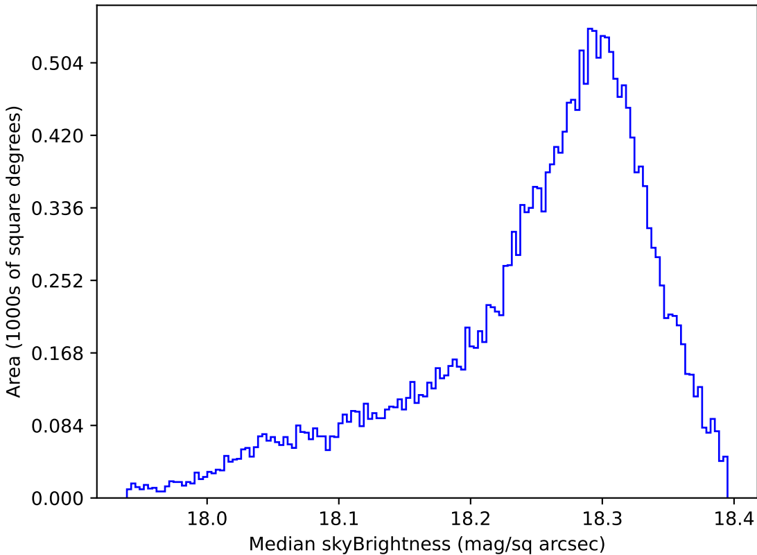
too_100_1v3.4_10yrs All sky y band: Median skyBrightness
