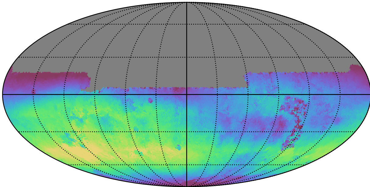
too_100_1v3.4_10yrs All sky u band: Median skyBrightness
