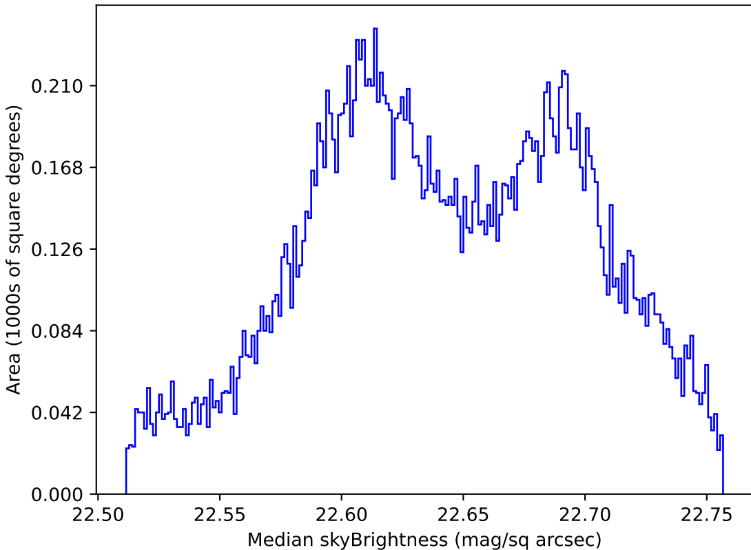
too_100_1v3.4_10yrs All sky u band: Median skyBrightness
