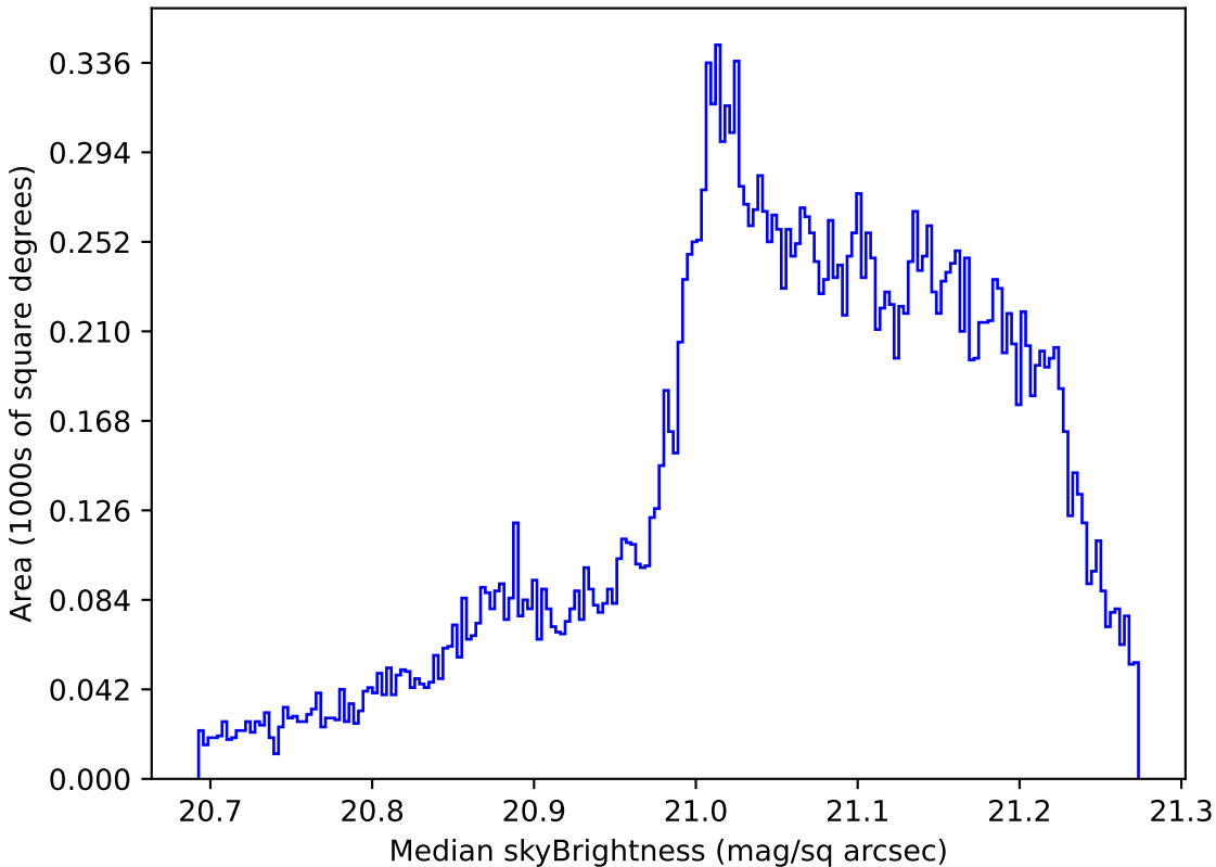
too_100_1v3.4_10yrs All sky r band: Median skyBrightness
