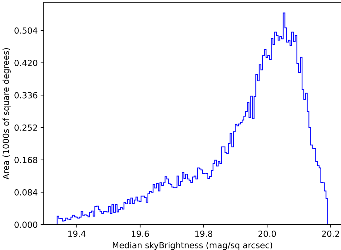
too_100_1v3.4_10yrs All sky i band: Median skyBrightness
