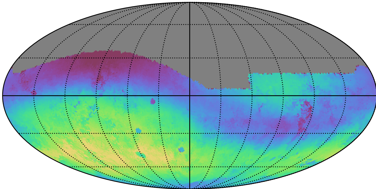
too_100_1v3.4_10yrs All sky g band: Median skyBrightness
