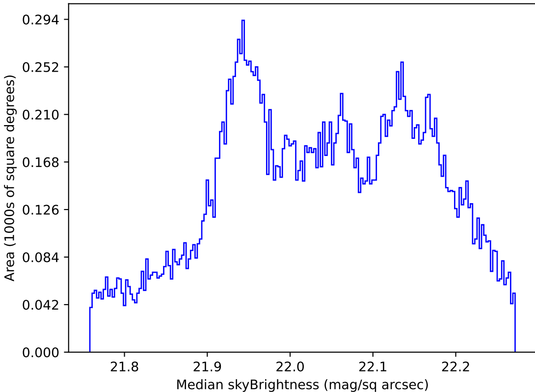
too_100_1v3.4_10yrs All sky g band: Median skyBrightness
