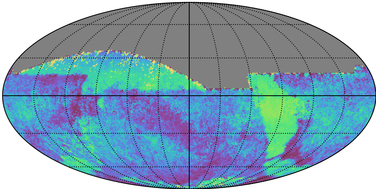
too_100_1v3.4_10yrs All sky all bands: Median skyBrightness
